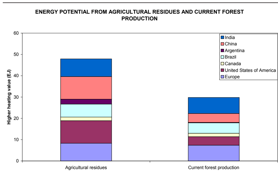
Figure 5. Higher heating value (HHV) of agricultural residue potentials and current forest production.
